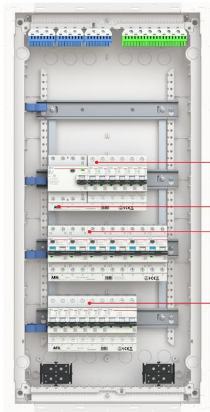
FN Residual current Circuit Breakers (RCCB) 4P, 2P
